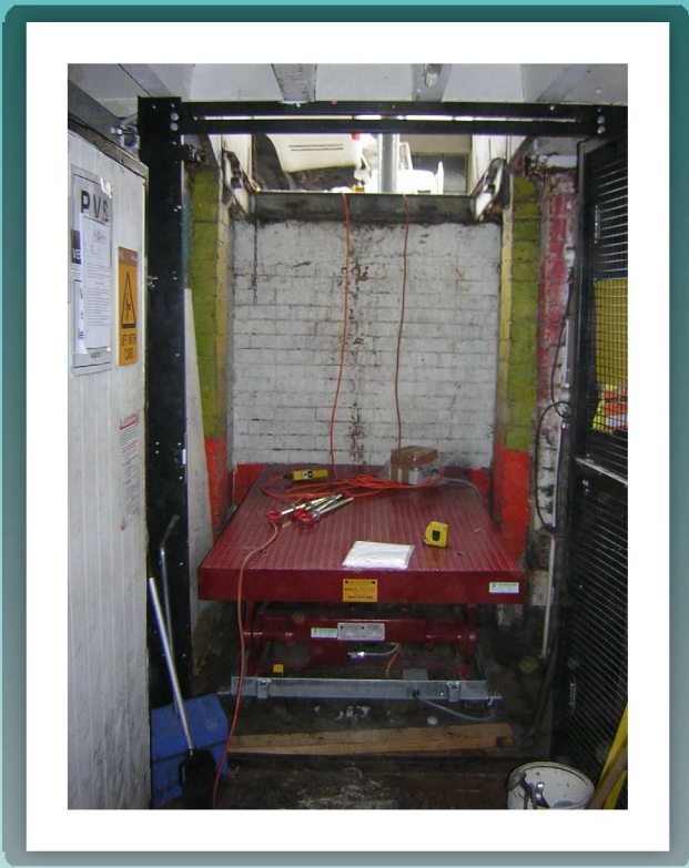
Installed. An interlocking gate system was integrated into this installation to eliminate personnel access to the pit when the table is in use.
